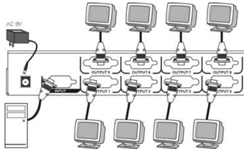
Figure 3 : 169363 Connection
